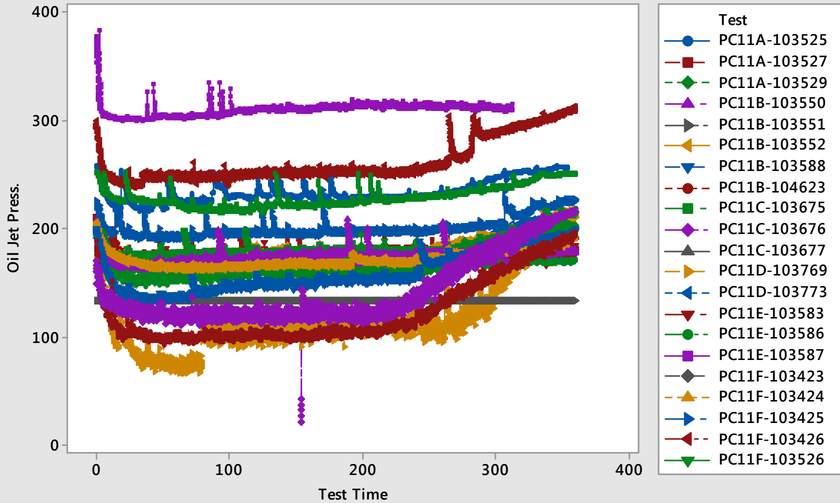
Scatterplot of Oil Jet Press. vs Test Time
