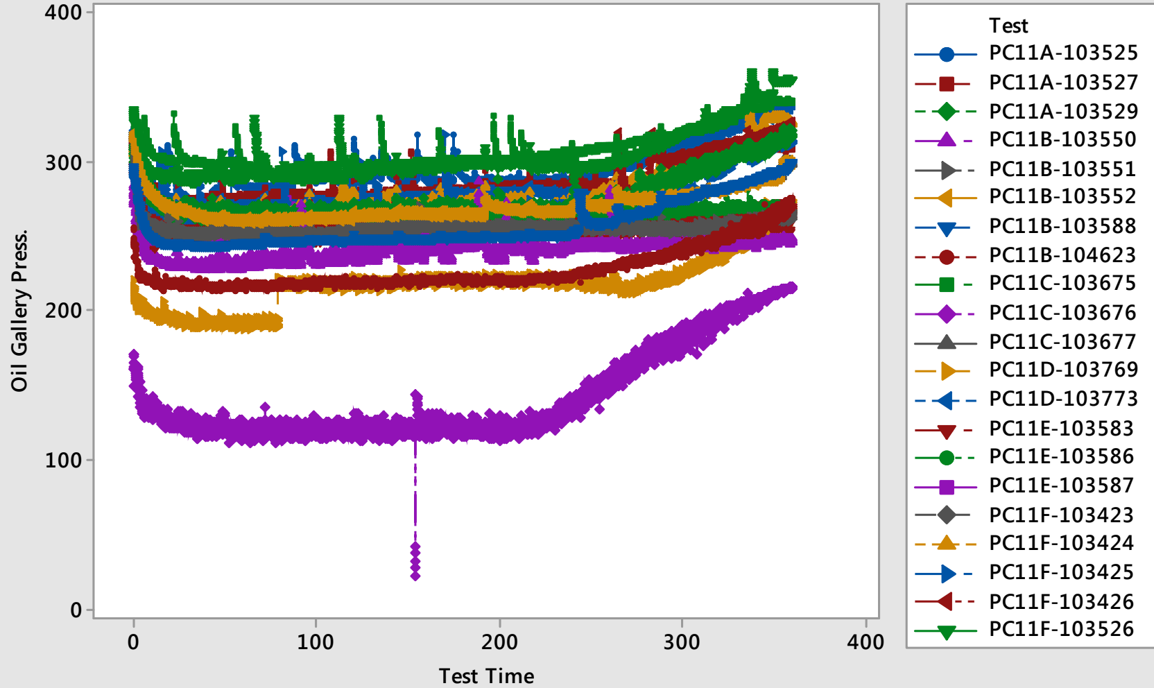
Scatterplot of Oil Gallery Press. vs Test Time
