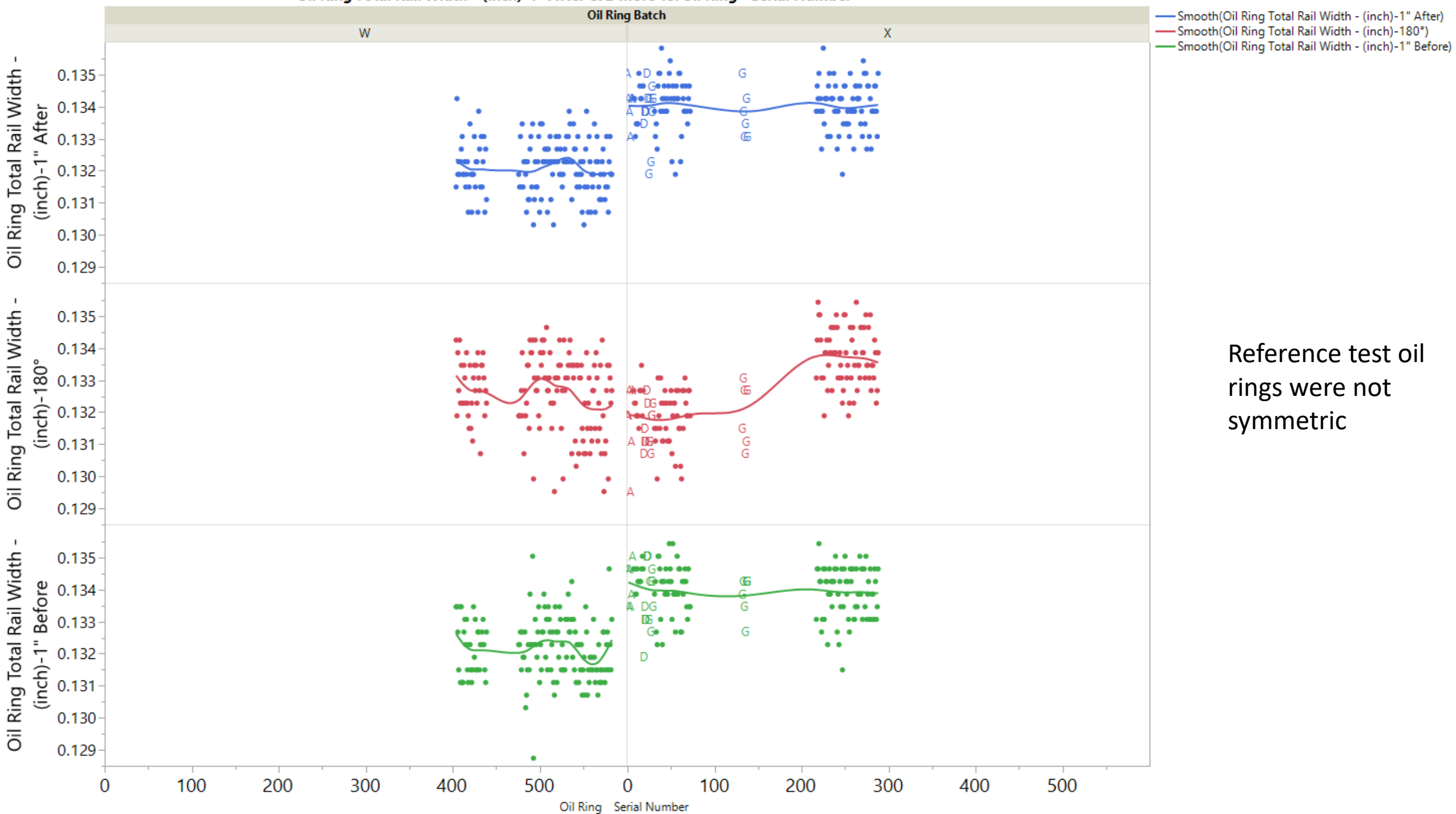
Oil Ring Total Rail Width - (inch)-1" After &amp; 2 more vs. Oil Ring Serial Number
