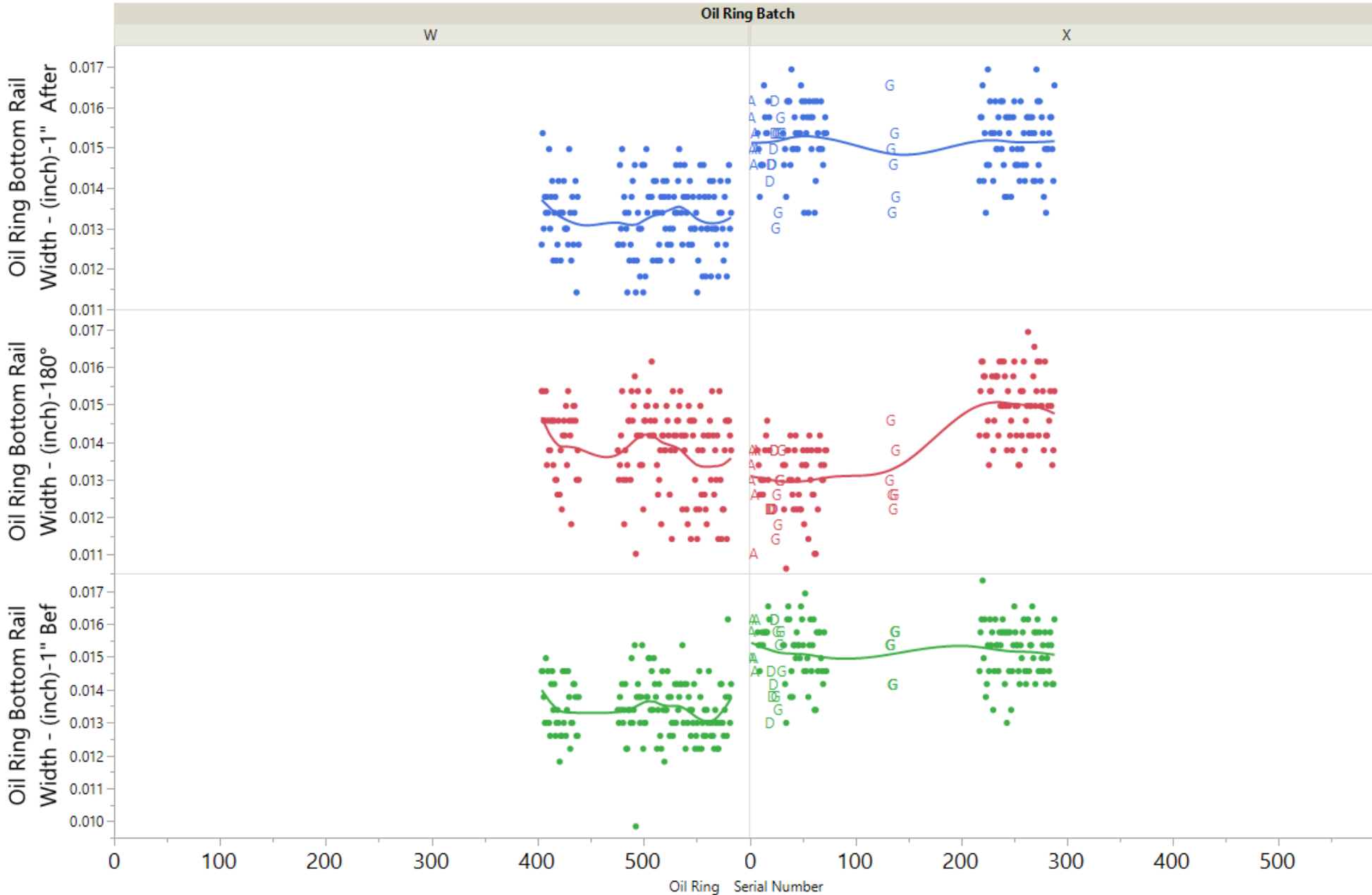
Oil Ring Bottom Rail Width - (inch)-1" Bef & 2 more vs. Oil Ring Serial Number
